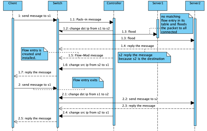
Fig. 3. Sequence diagram of redirecting
