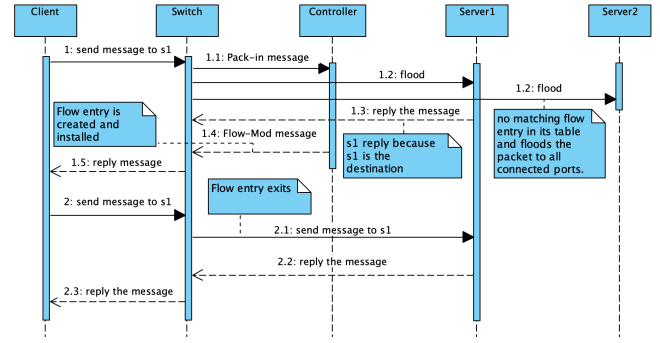
Fig. 2. Sequence diagram of forwarding
