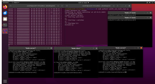
Fig. 5. Test Result of Task 1
