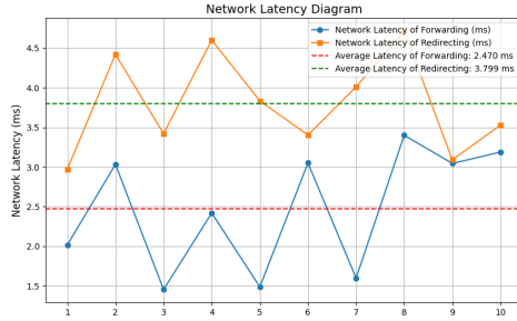
Fig. 10. Network Latency Diagram
