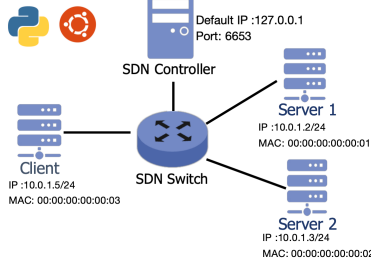
Fig. 1. The network topology
