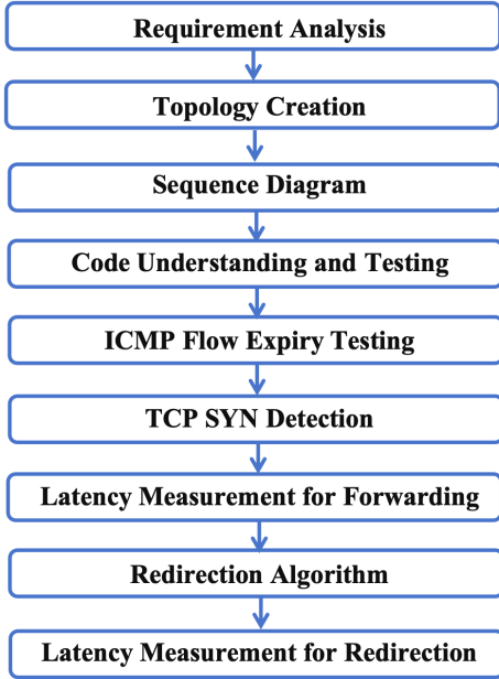
Fig. 4. Flowchart of Implementation
